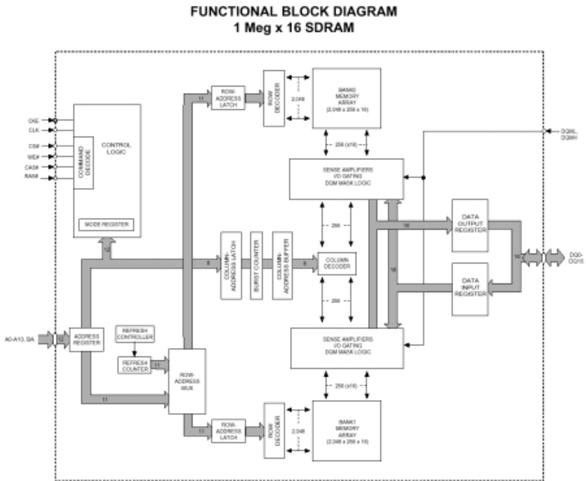
Figure 15 MICRON's 16Mbit SDRAM Block Diagram
