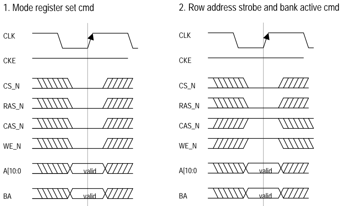
Figure 15.1-1 Timing Diagrams of basic commands for SDRAM control
