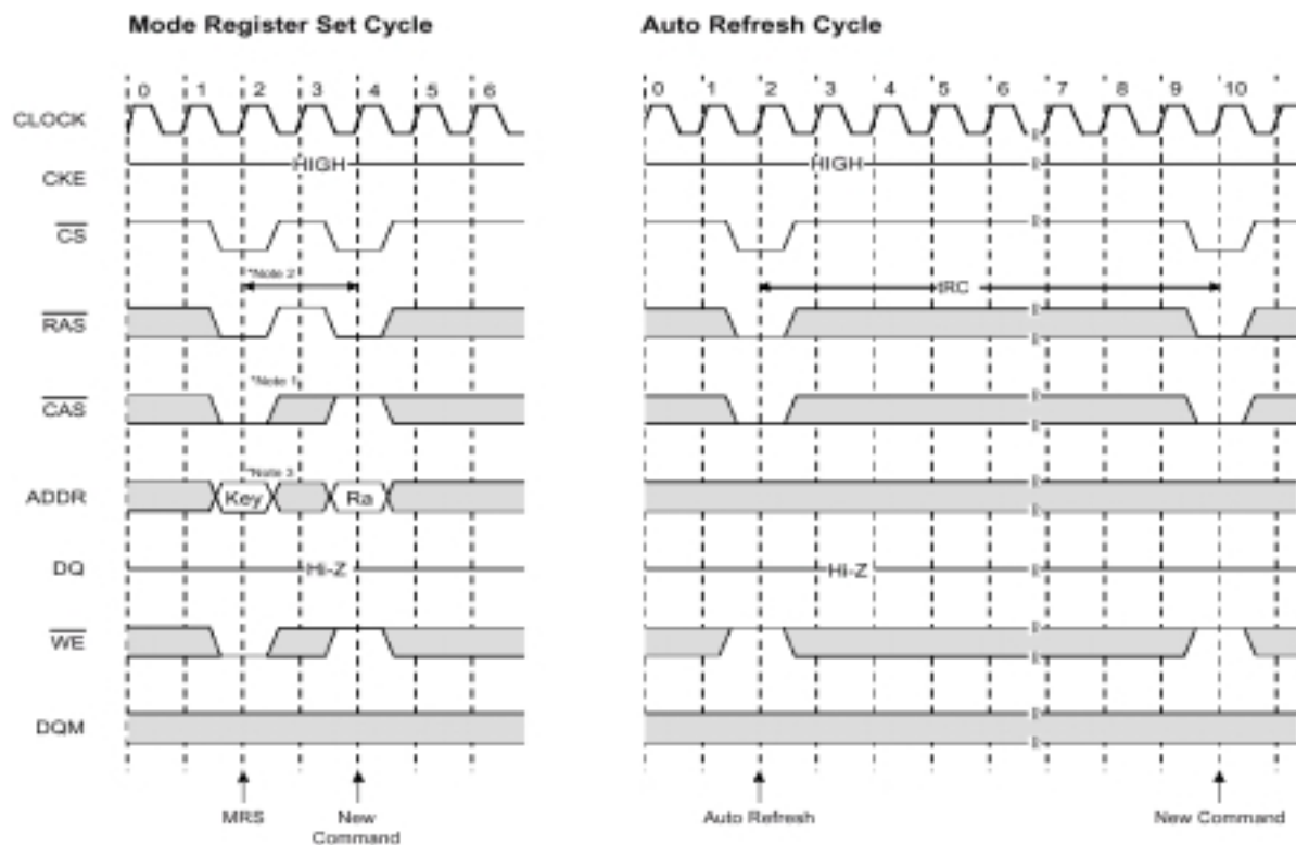
Figure 15.2-2 Timing Diagrams of mode register set and auto refresh cycle (Samsung SDRAM)
