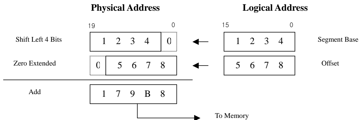
Figure 4.3 Physical Address Generation
