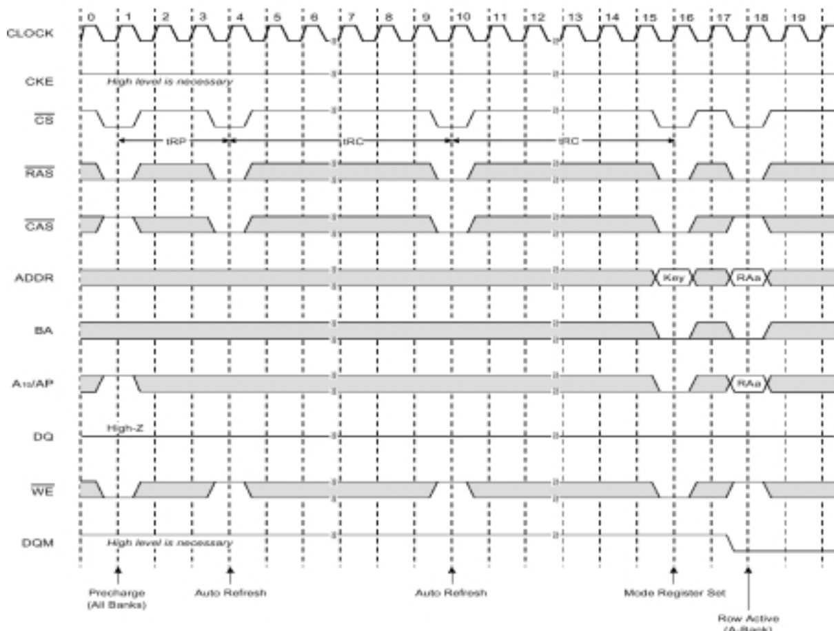
Figure 15.2 Timing Diagrams of Power-Up Sequence (Samsung SDRAM)
