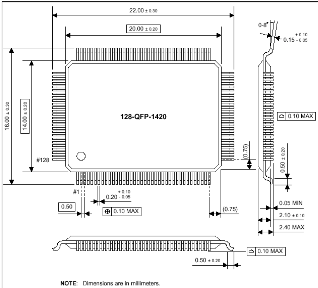
Figure B.2 Physical Dimension
