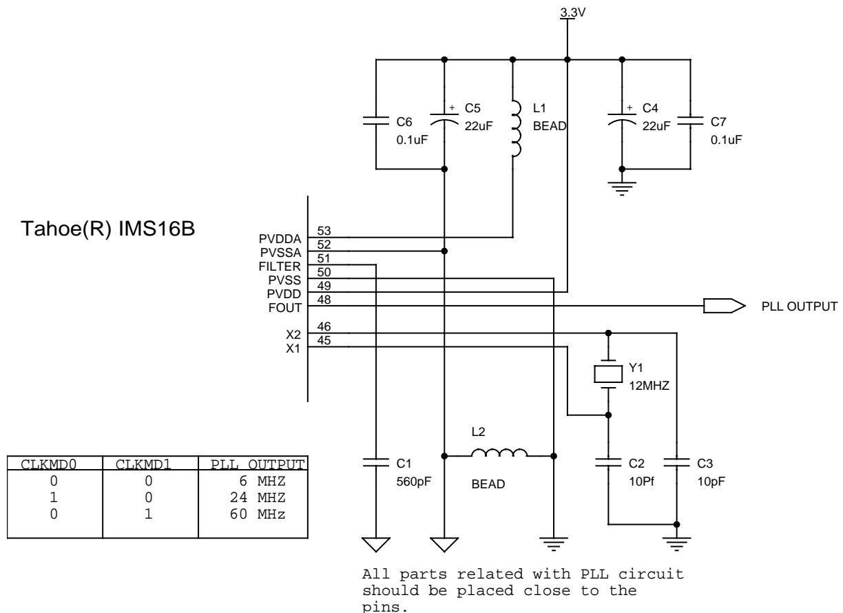
Figure C.2 Example circuit for PLL Frequency Synthesizer
