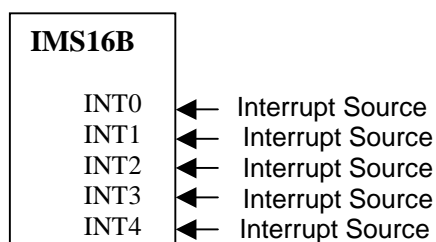
Figure 9.5 Fully Nested Mode Interrupt Controller Connections
