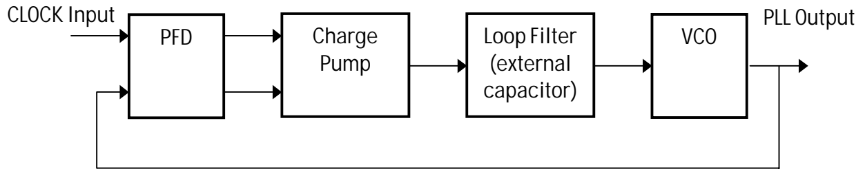
Figure C.1 Main Component of PLL Frequency Synthesizer
