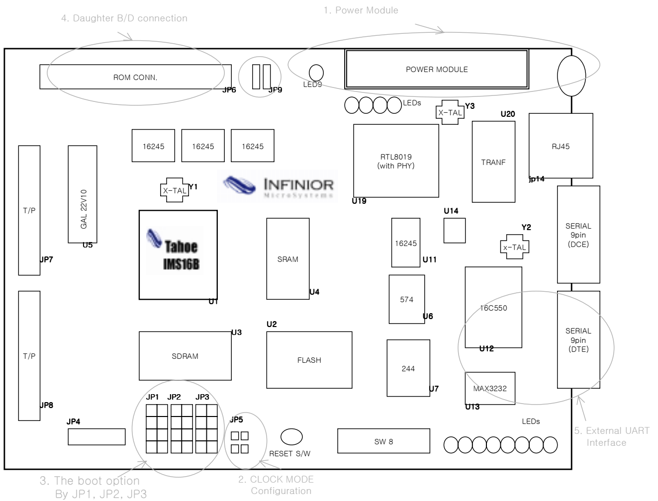
Figure C-8 Tahoe ® IMS16B Evaluation Board2 Layout
