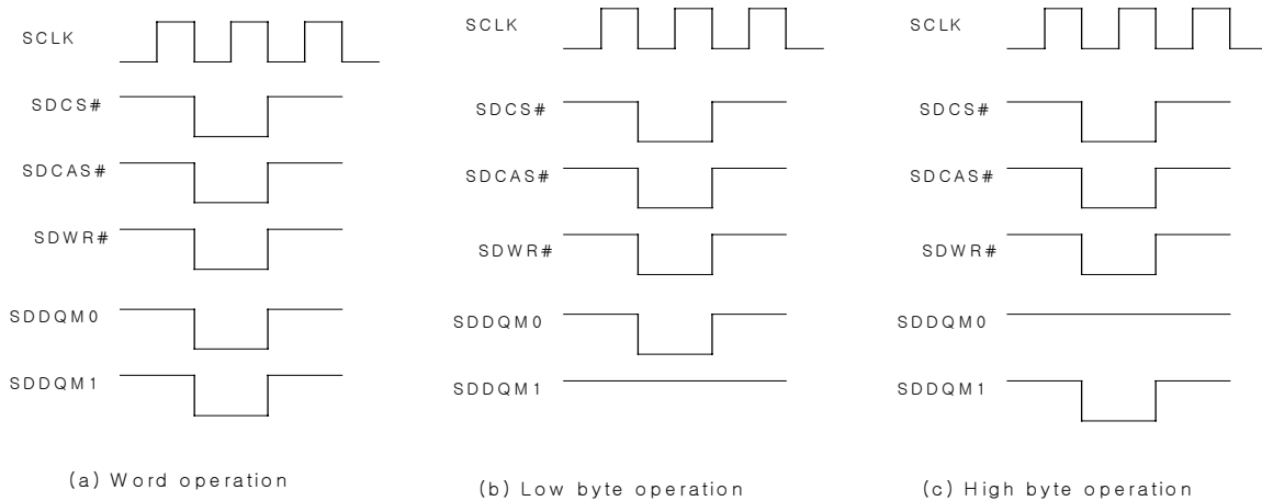
Figure 15.7.1 Normal Word and Byte Operation Timing
