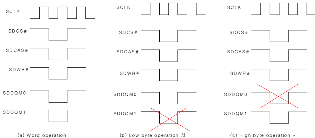
Figure 15.7.2 IMS16B – Only word operation
