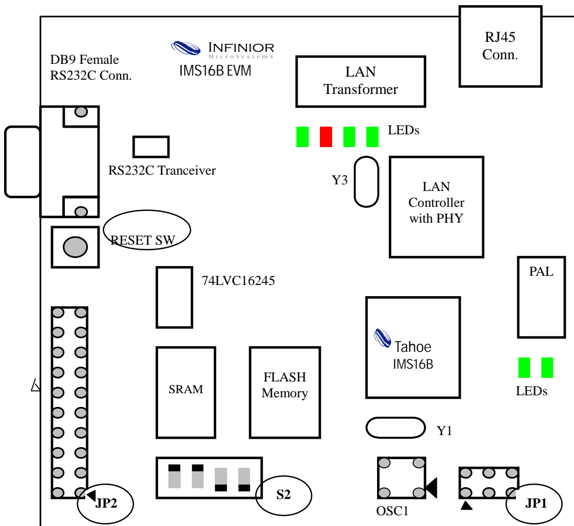
Figure C.4 Tahoe® IMS16B Evaluation Board1 Layout
