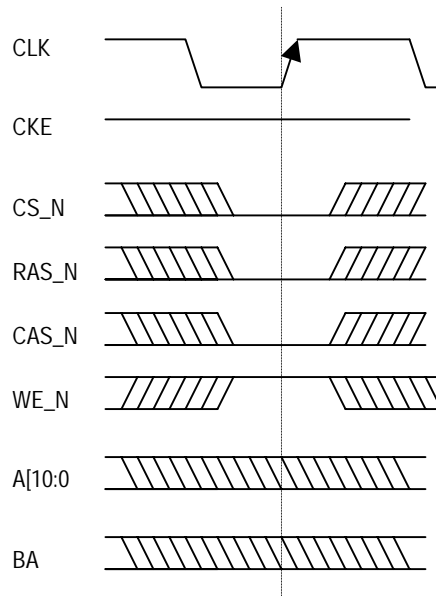
Figure 15.1-1 Timing Diagrams of basic commands for SDRAM control(Contd)
